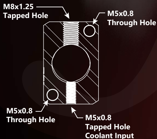
Tool Holder CIT-SAU919-S-CT
