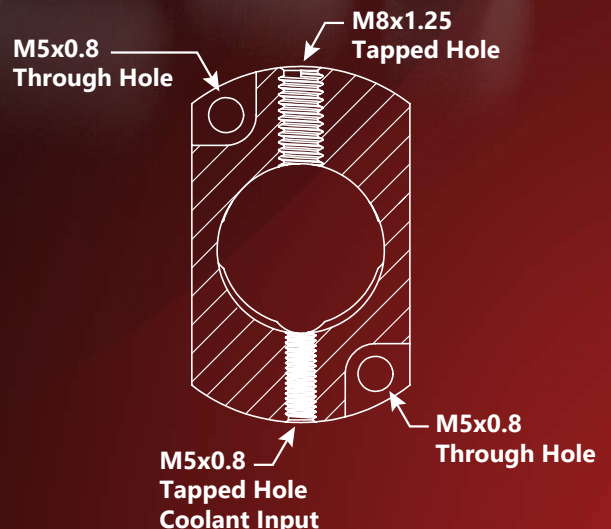
Tool Holder CIT-SAU825-S-CT
